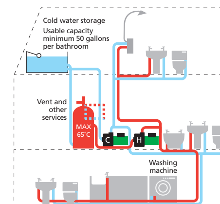
Figure 17: Super booster whole house systems
