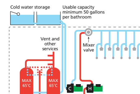
Figure 18: Super booster to multiple showers
