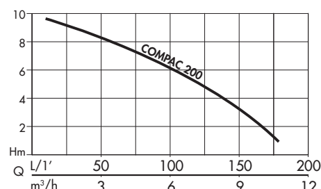
PERFORMANCE CURVE
